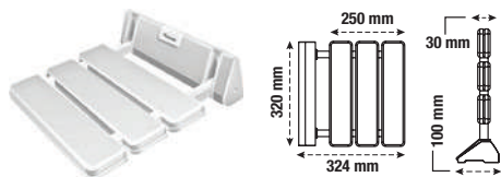
Chair/Stool Foldable (Wall Mounted)
