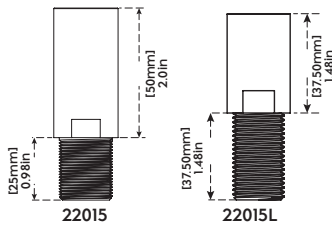
Extension Nipple
