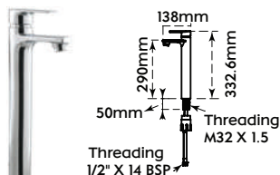
Single Lever Basin Mixer - 12" High
