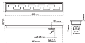
Shower Channel Drain - C Square
