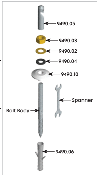
Rack Bolt Accessories Set (without Bolt)
