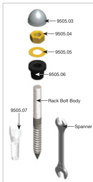
Breakup view of 9505 parts
