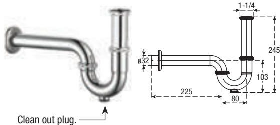
P Trap
