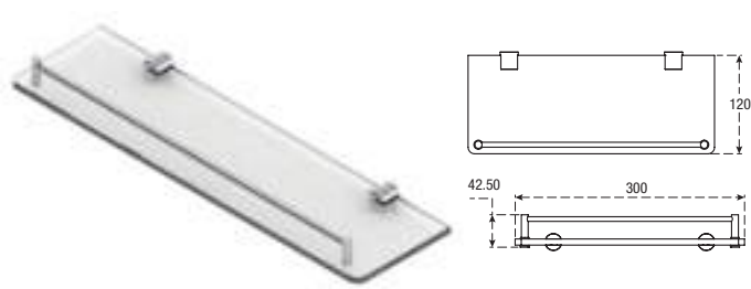
Glass Shelf with Rail-H 2 O
