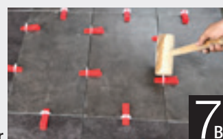
Or simply Remove Wedges with a Mallet
