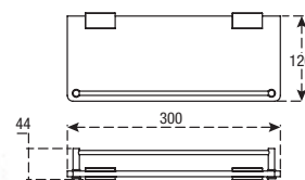
Glass Shelf with Rail-Rectangular (Wall Brackets)
