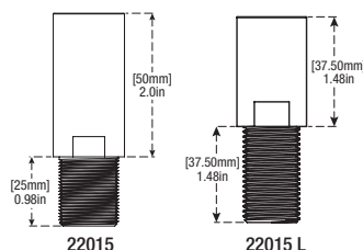
Designed for West Bengal Both Thread 37mm Long
