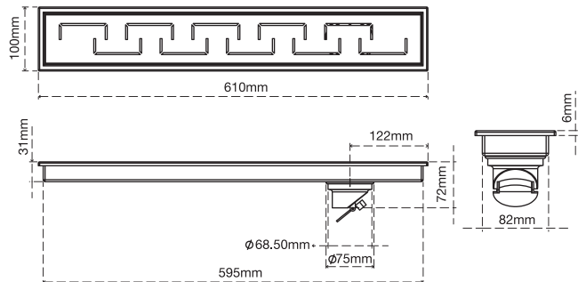
Shower Channel Drain - C Square
