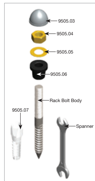
Breakup view of 9505 parts
