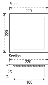
Dustbin Cover Counter Mounted
