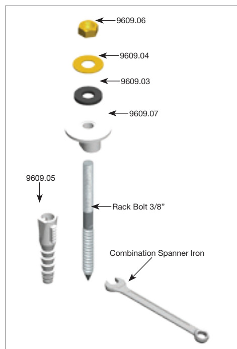
Breakup view of 9609 parts
