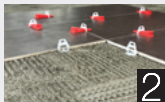
Tile Spacer below the one Tile
