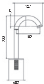
Pillar Cock Touch On-Touch Off (Swan Neck) (Fits all counter top basins)
