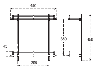
Double Shelf-Rectangular
