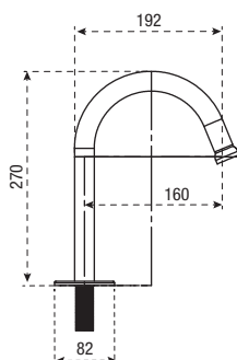
Pillar Cock Touch On OFF for Counter Top Basins (Fits all counter top basins)
