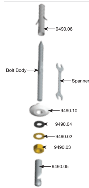
Breakup view of 9490 parts
