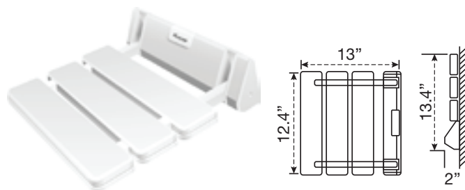
Chair/Stool Foldable (Wall Mounted)
