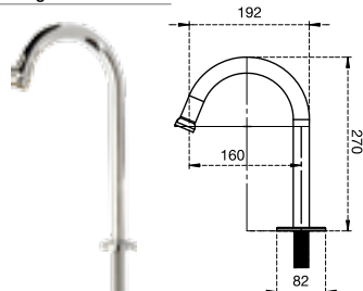
Pillar Cock Touch On - Touch Off (Swan Neck) (Fits all counter top basins)
