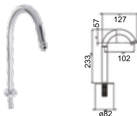
Pillar Cock Touch On - Touch Off (Swan Neck)
