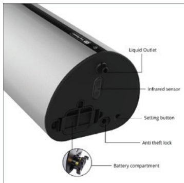
Automatic (Sensor) Lotion Dispenser Silver
