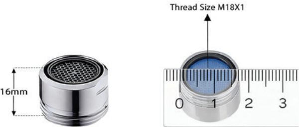
Aerator Foam Flow (Outer Thread )
