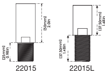
Extension Nipple
